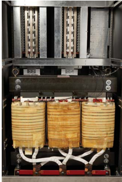
K13-rated transformer, coupled with a 200%-rated neutral standard with upgrades available.
